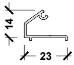
APW.BAY.021 BAY POLE NEST (STANDARD)
