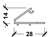
APW.BAY.022 BAY POLE NEST (FLUSH)
