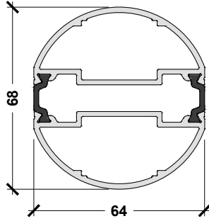
ACW81.772 BAY POLE (UNIVERSAL)
