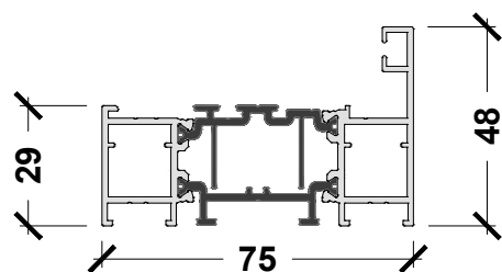
APX.SRS.048 48MM SINGLE REBATE STANDARD
