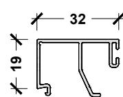
APX.GLB.011 GLAZING BEAD 1
