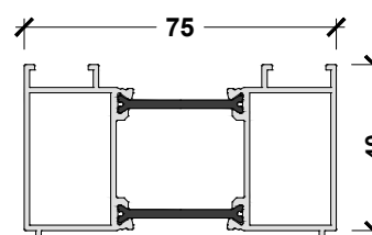
APX.ANC.210 40MM ADD-ON (STANDARD)
