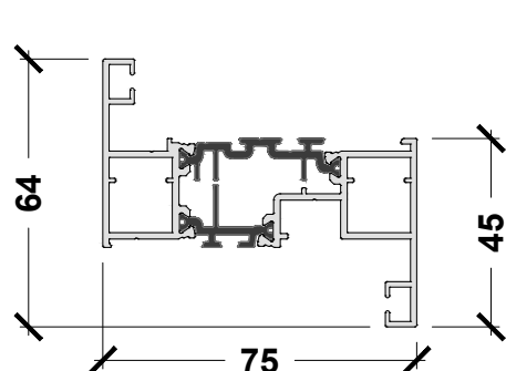
APW.TTS.064 64MM TILT TURN SASH
