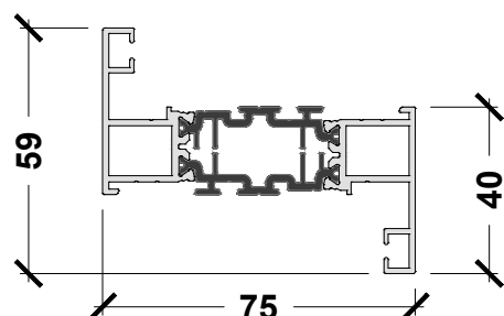
APW.DRZ.059 59MM DOUBLE REBATE Z
