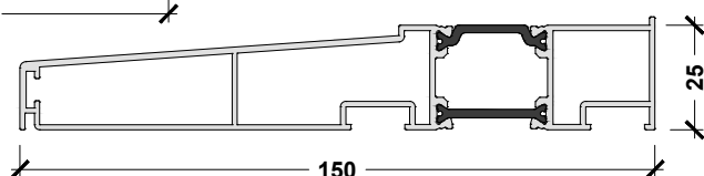
APX.OPC.150 150MM CILL
