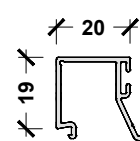
APX.GLB.021 GLAZING BEAD 2
