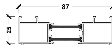
APX.ANC.220 25MM ADD-ON (FLUSH)
