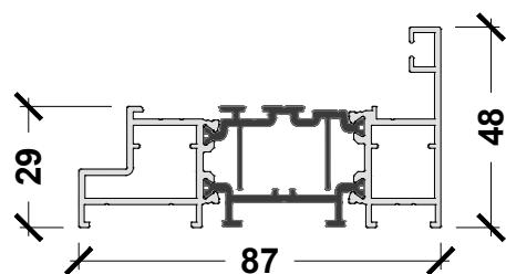
APW.SRF.048 48MM SINGLE REBATE FLUSH
