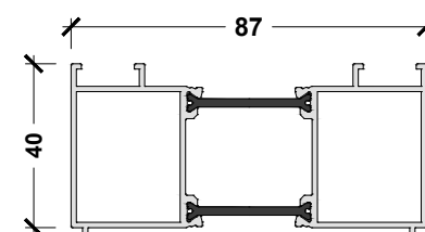
APX.ANC.230 40MM ADD-ON (FLUSH)
