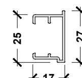
APX.ANC.072 25MM CLIP ON TRIM (UPSTAND)
