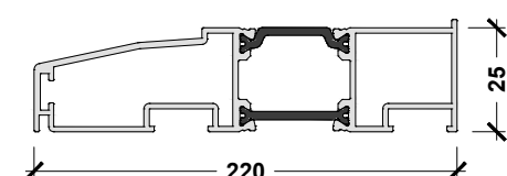
APX.CIL.150 220MM CILL NOSE
