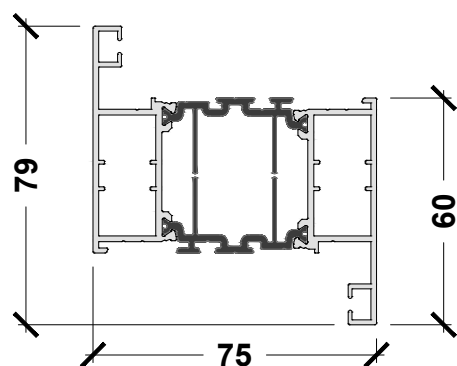
APW.DRZ.079 79MM DOUBLE REBATE Z
