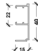
APX.ANC.081 40MM CLIP ON TRIM
