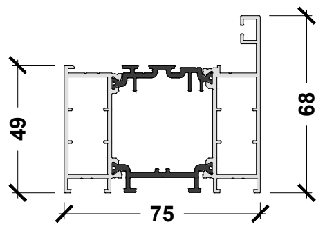
APX.SRS.068 68MM SINGLE REBATE STANDARD
